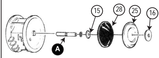
Shaft Assembly with back-up diaphragm
