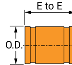
Fig. 7080 Adapter Nipple (GR x GR)
